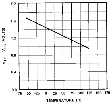
VTH - V1C vs TEMPERATURE
