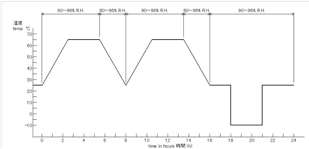
Humidity-Temperature Cycle
