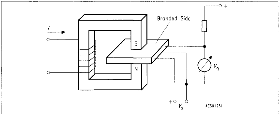
Figure 81 Sensor/Magnetic-Field Configuration
