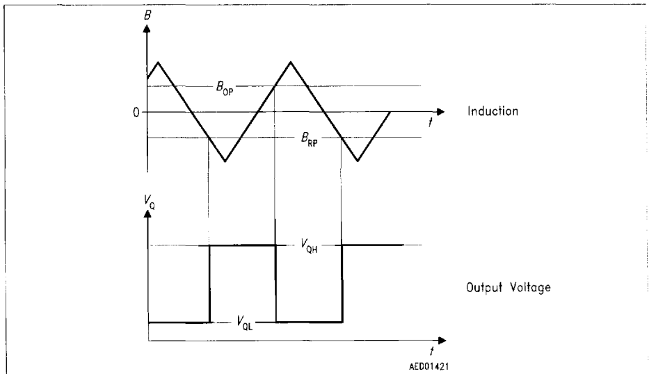
Figure 82 Switching Characteristics Bipolar Type
