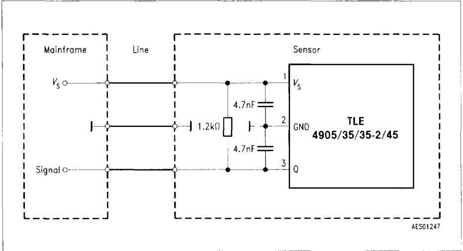
Figure 84 Application Circuit
