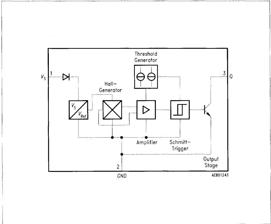
Figure 78 Block Diagram
