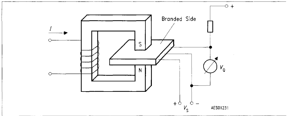
Figure 79 Sensor/Magnetic-Field Configuration
