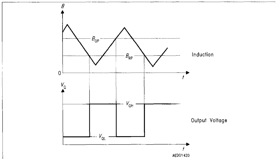
Figure 80 Switching Characteristics Unipolar Type
