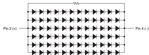
5700K Cool White 12 Series x 6 Parallel = 72 LEDs
