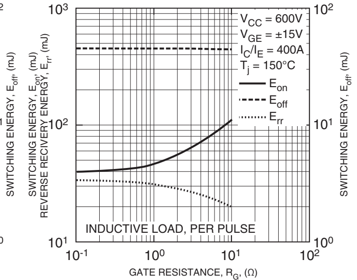
HALF-BRIDGE SWITCHING CHARACTERISTICS (TYPICAL)
