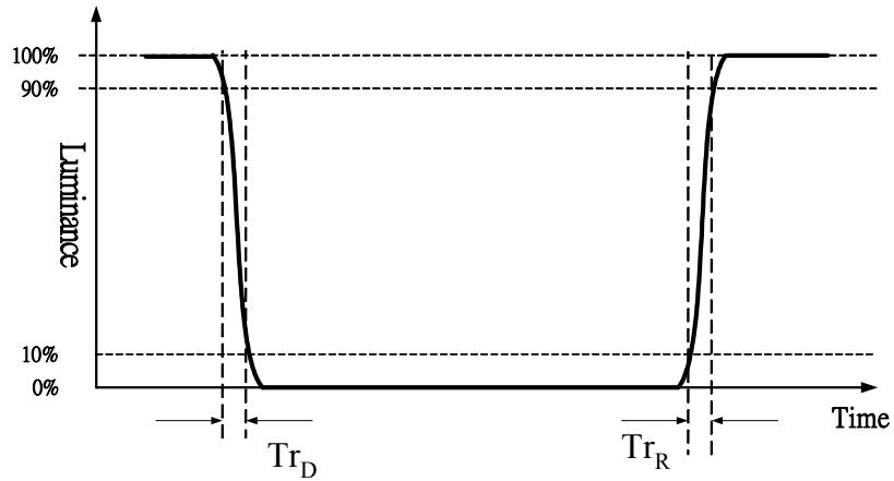
Fig.4-4 Response time
