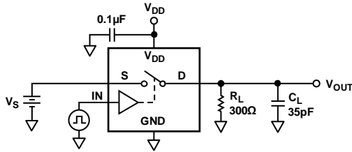
Figure 17. Switching Times
