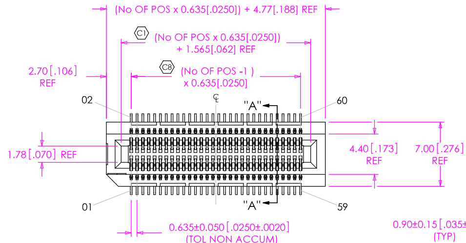
FIG. 1 -LC OPTION SHOWN MEC6-130-02-X-DV-LC SHOWN (FOR POSITIONS -10, -20, -30 & -40)
