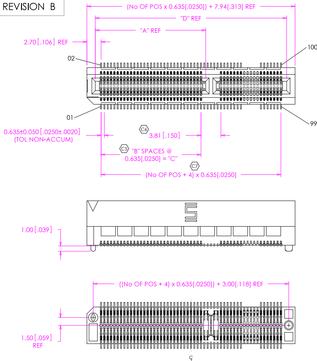
FIG. 2 MEC6-150-02-X-DV-A SHOWN FOR POSITIONS -50 THRU 70 (SAME AS FIG. 1, UNLESS OTHERWISE STATED)
