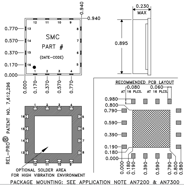
Package # 273LF
