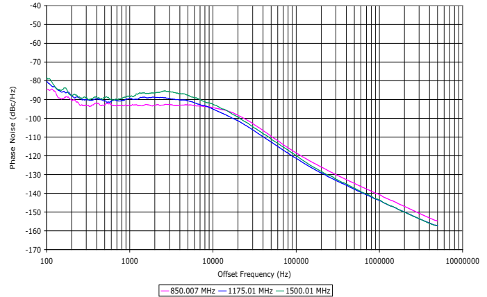
Phase Noise
