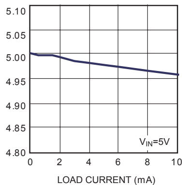
LDO Load Regulation
