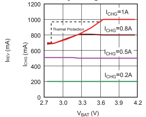
Charge Current vs Battery Voltage
