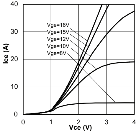
Fig. 20 - Typical IGBT Output Characteristics T_J = 25^\circ\text{C} ; t_p = 80 \mu\text{s}
