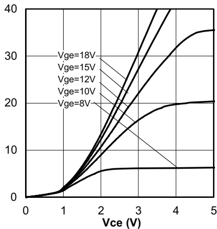
Fig. 21 - Typical IGBT Output Characteristics T_J = 125^\circ\text{C} ; t_p = 80 \mu\text{s}
