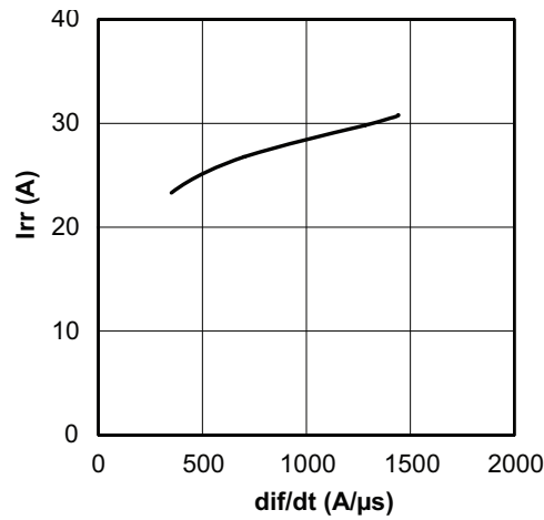
Fig. 15 - Typical Diode I_{RR} vs. df/dt V_{CC} = 300\text{ V} ; V_{GE} = 15\text{ V} ; I_F = 10\text{ A} ; T_J = 125^\circ\text{C}
