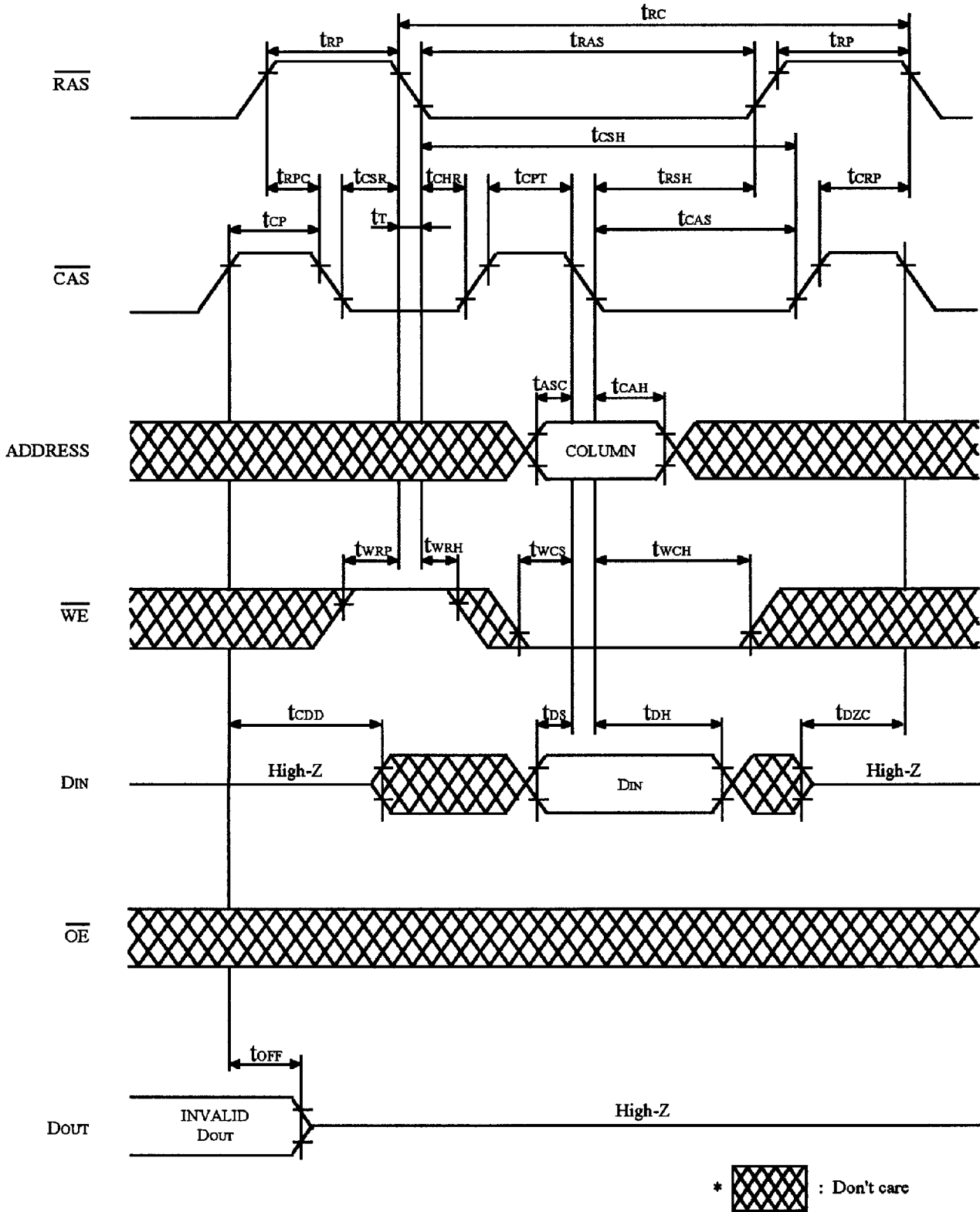
FIGURE 18. \overline{CAS} BEFORE \overline{RAS} REFRESH COUNTER CHECK CYCLE (WRITE)
