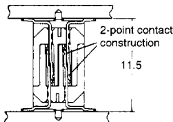
11.5mm type
