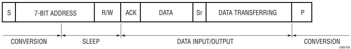
Figure 4. Conversion Sequence
