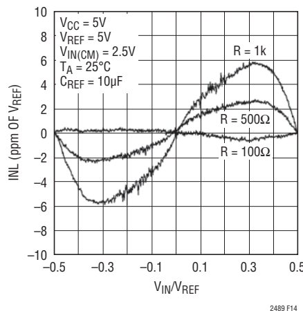
Figure 14. INL vs Differential Input Voltage and Reference Source Resistance for C_{REF} > 1\mu\text{F}
