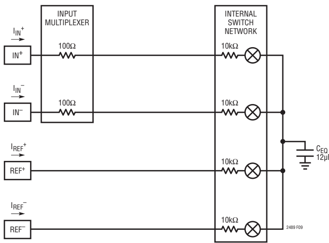
Figure 9. Equivalent Analog Input Circuit
