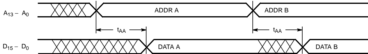
Read Operation Timing Diagram [6]
