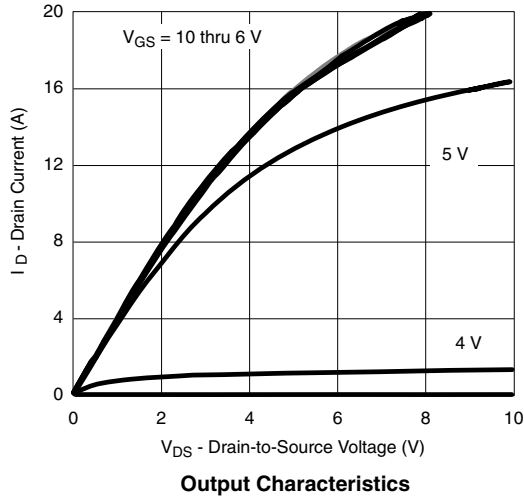
Output Characteristics
