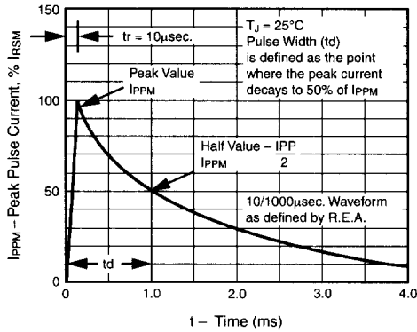
Fig. 3 – Pulse Waveform
