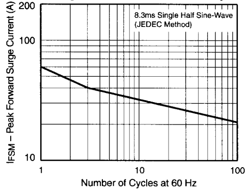
Fig. 4 - Maximum Non-Repetitive Forward Surge Current Uni-Directional Only
