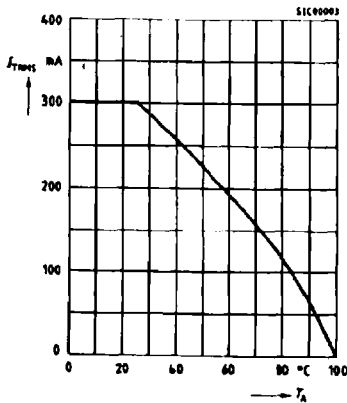
Current reduction I_{TRMS} = f(T_A) , R_{thJA} = 125 K/W SiTAC switch soldered in PCB or base plate
