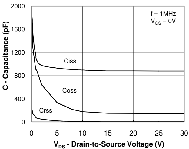
Fig.5 Capacitance Characteristic
