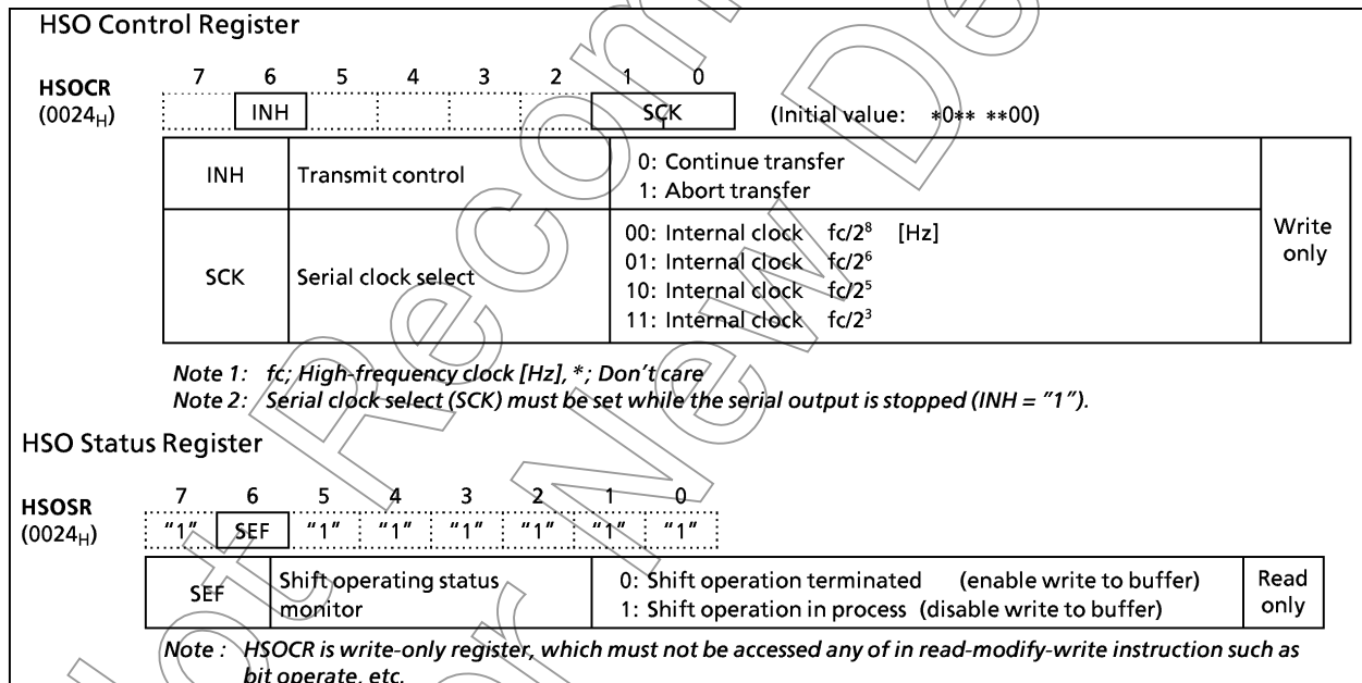
Figure 2-39. HSO Control Register and Status Register
