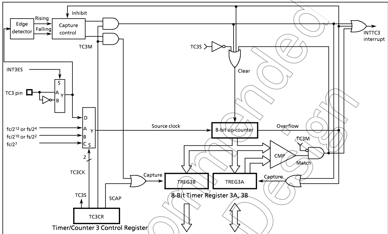
Figure 2-22. Timer/Counter 3
