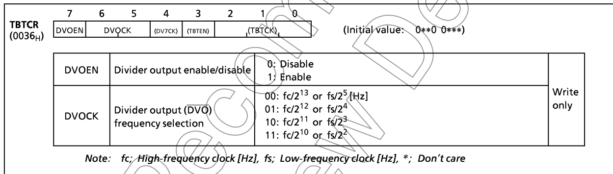
Figure 2-14. Divider Output Control Register
