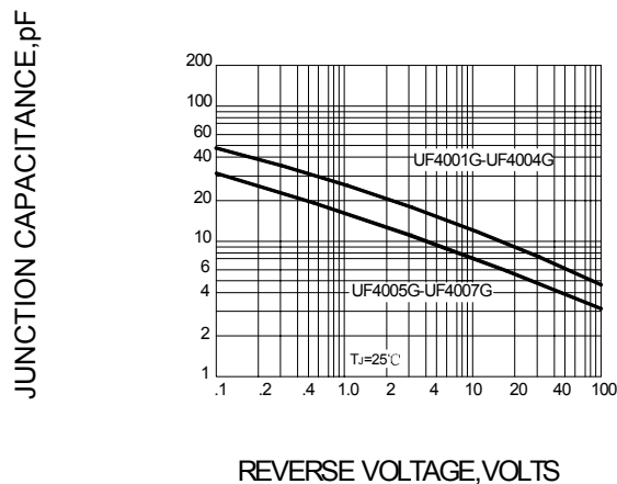
FIG.5–TYPICAL JUNCTION CAPACITANCE
