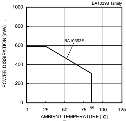
Fig.24 Derating Curve
