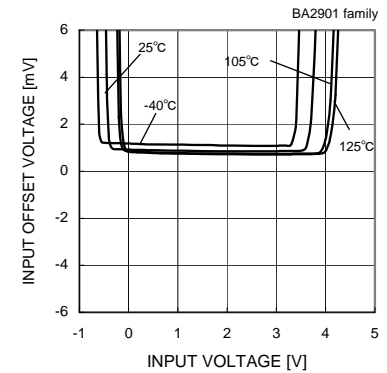
Fig.104 Input Offset Voltage - Input Voltage (VCC=5V)
