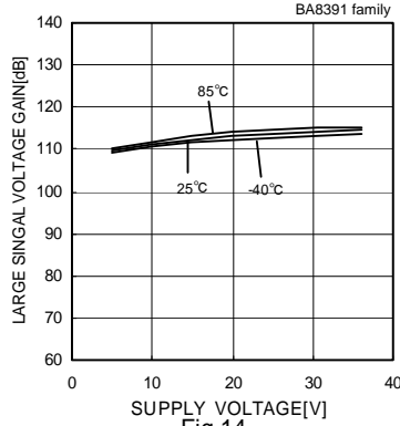
Large Signal Voltage Gain - Supply Voltage
