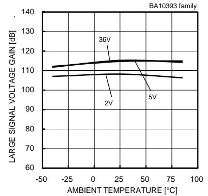
Fig.38 Large Signal Voltage Gain - Ambient Temperature
