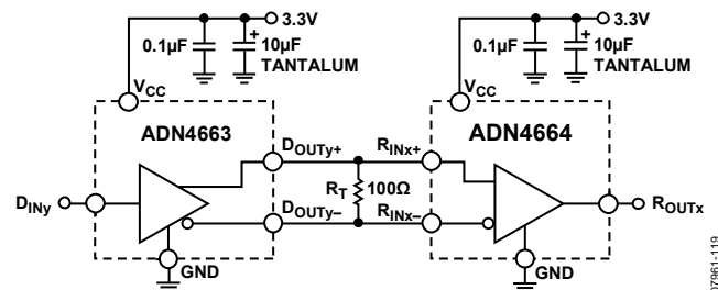
Figure 23. Typical Application Circuit
