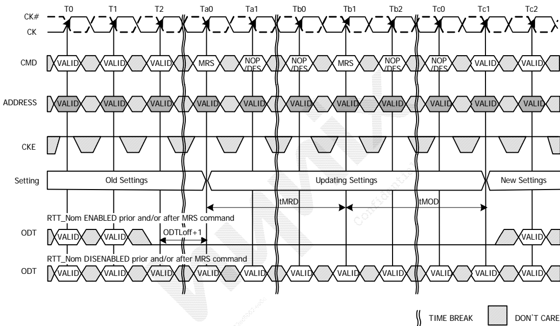
Figure 4. t_{MRD} Timing
