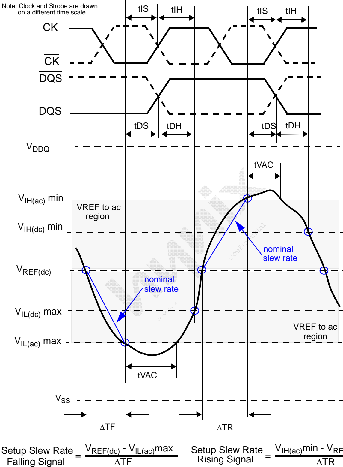
Figure 3 - Illustration of nominal slew rate and t_{VAC} for setup time t_{DS} (for DQ with respect to strobe) and t_{IS} (for ADD/CMD with respect to clock).
