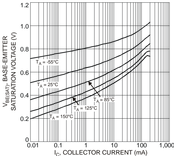
Fig. 7 Base-Emitter Saturation Voltage vs. Collector Current
