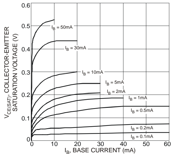
Fig. 4 Typical Collector-Emitter Saturation Voltage vs. Base Current
