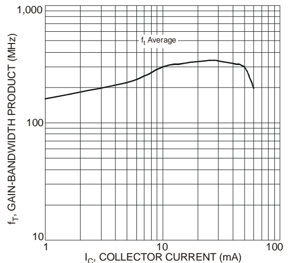
Fig. 10 Typical Gain-Bandwidth Product vs. Collector Current
