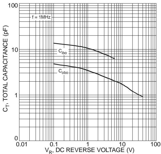
Fig. 9 Total Capacitance vs. Reverse Voltage
