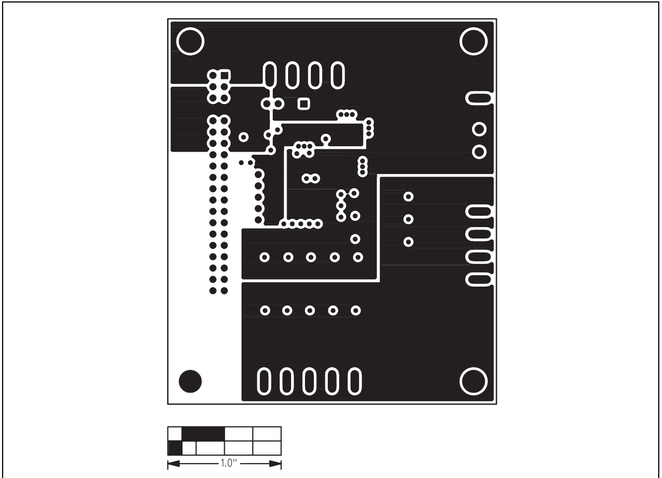
Figure 6. MAX1168 EV Kit PC Board Layout—Inner Layer 3 (VDD)
