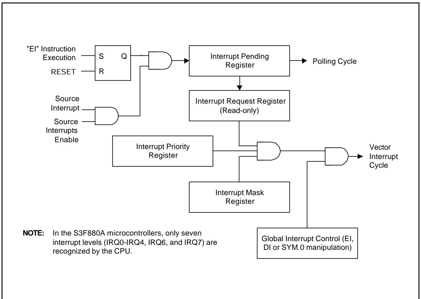
Figure 5-4. Interrupt Function Diagram
