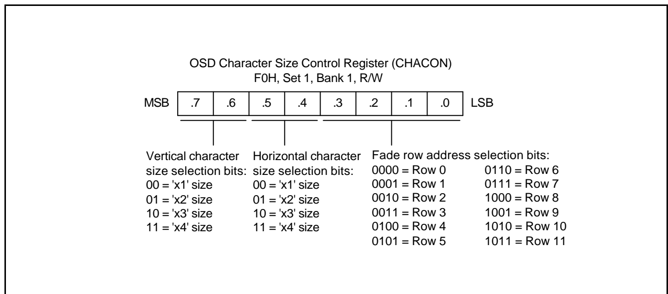
Figure 13-4. OSD Character Size Control Register (CHACON)
