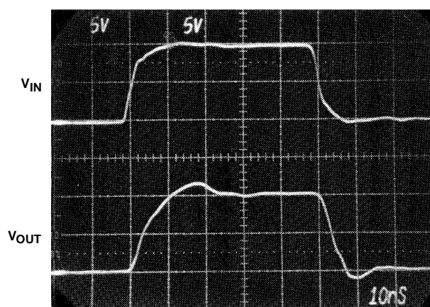
R_S = 50\Omega, R_L = 1k\Omega
