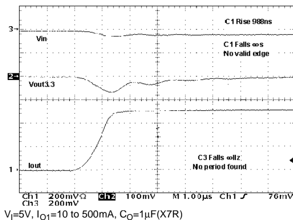
Figure 24 : Load Transient
