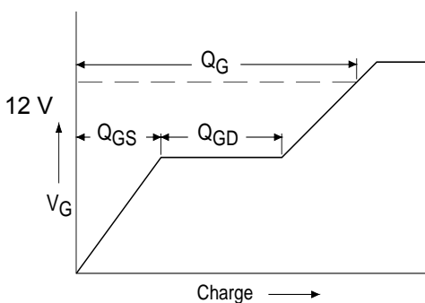
Fig 29a. Basic Gate Charge Waveform
