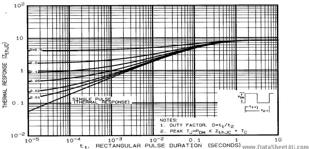
Fig 27. Maximum Effective Transient Thermal Impedance, Junction-to-Case
