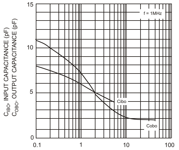
V_{CB} , COLLECTOR-BASE VOLTAGE (V) Fig. 6, Input and Output Capacitance vs. Collector-Base Voltage (NPN-4124)
