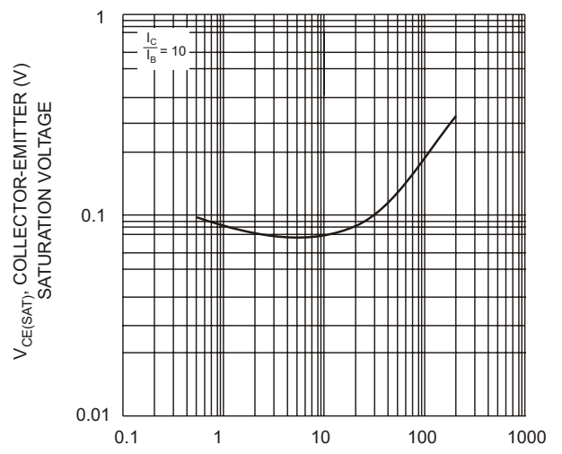
I_C , COLLECTOR CURRENT (mA) Fig. 8, Typical Collector-Emitter Saturation Voltage vs. Collector Current (NPN-4124)
