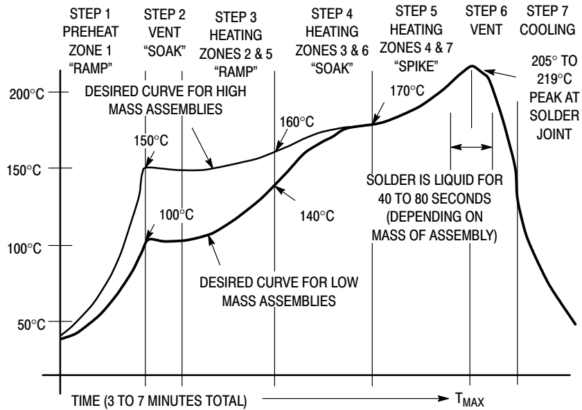
Figure 6. Typical Solder Heating Profile for D 2 PAK
