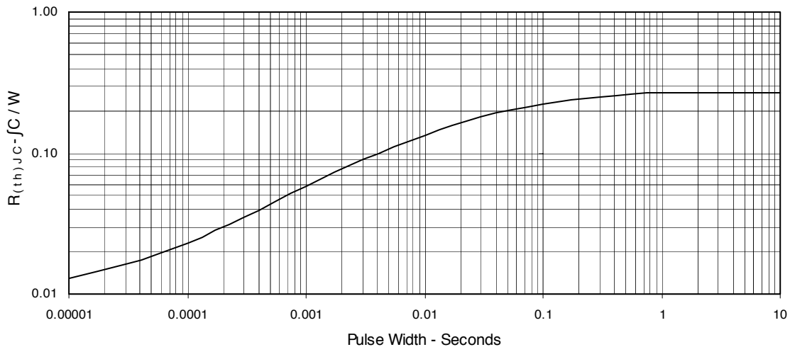
Fig. 12. Maximum Transient Thermal Resistance
