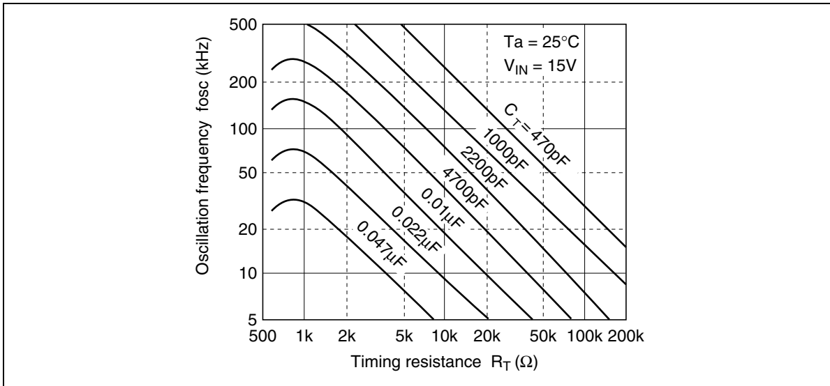
Figure 7 Oscillation Frequency vs. Timing Resistance
