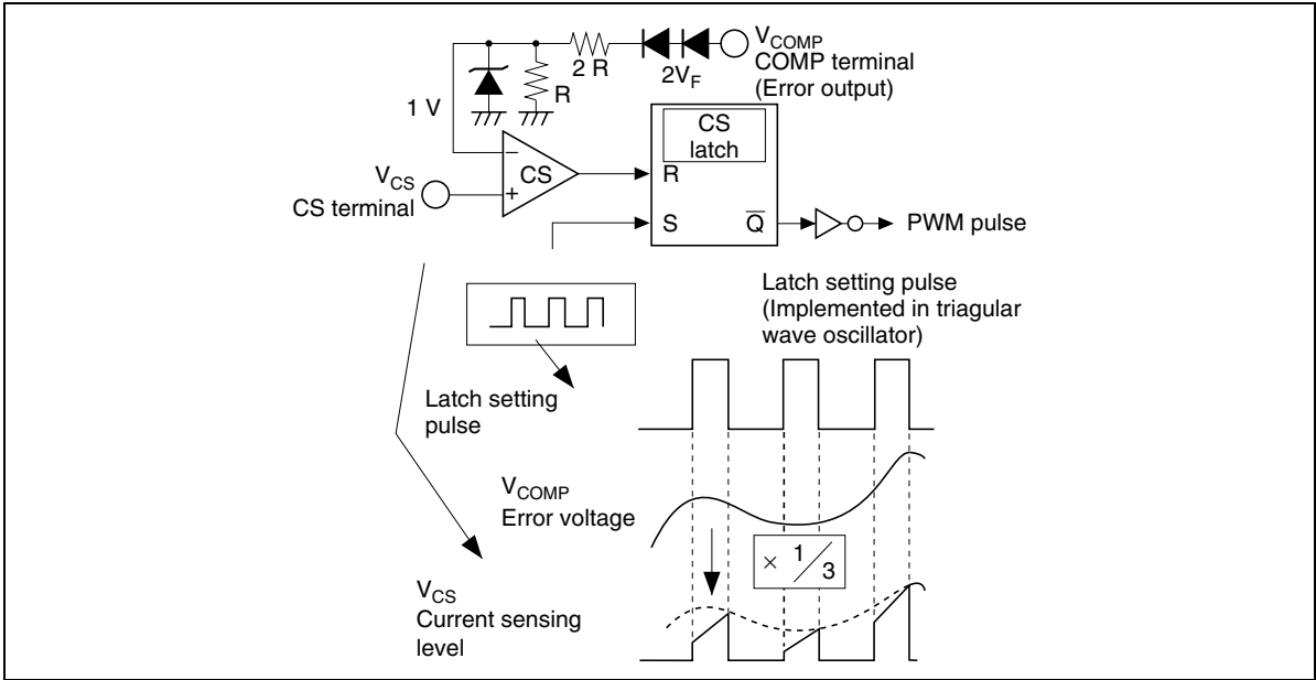
Figure 3 Operation Diagram of Current Sensing Part
