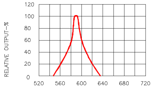
Fig.2 SPECTRAL RESPONSE
