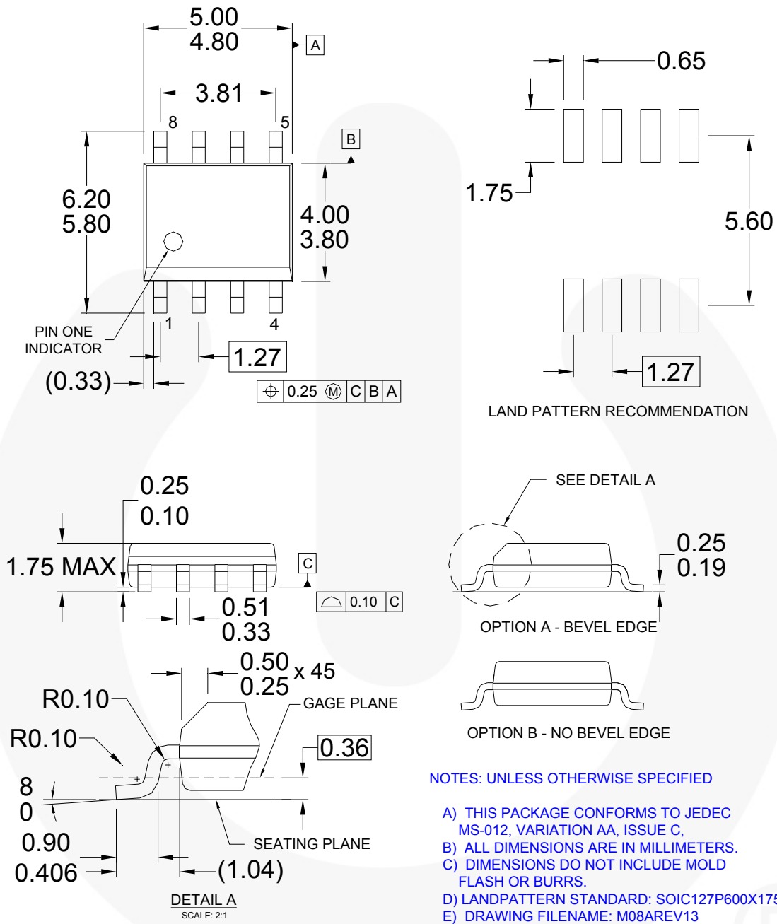
Figure 54. 8-Lead SOIC
