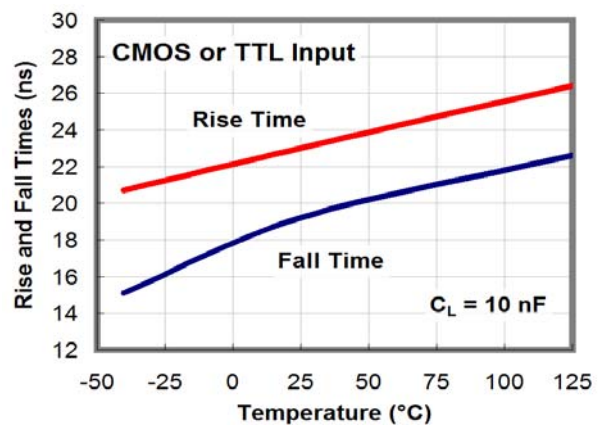
Figure 38. Rise and Fall Time vs. Temperature
