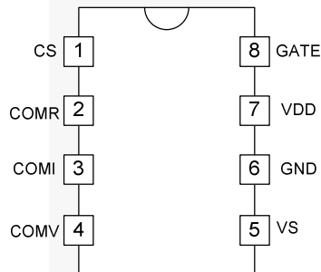
Figure 5. Pin Configuration
