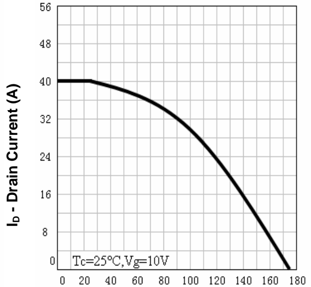
Drain Current
