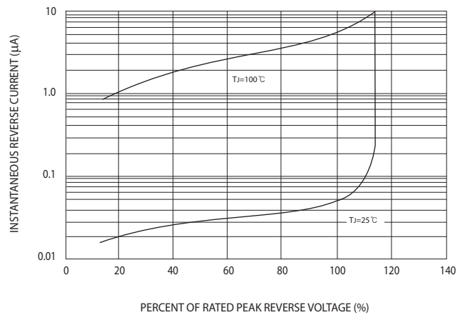
FIG.4-TYPICAL REVERSE CHARACTERISTICS
