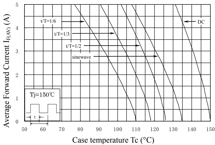
Current Derating
