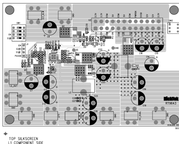
Figure 7. Component Side
