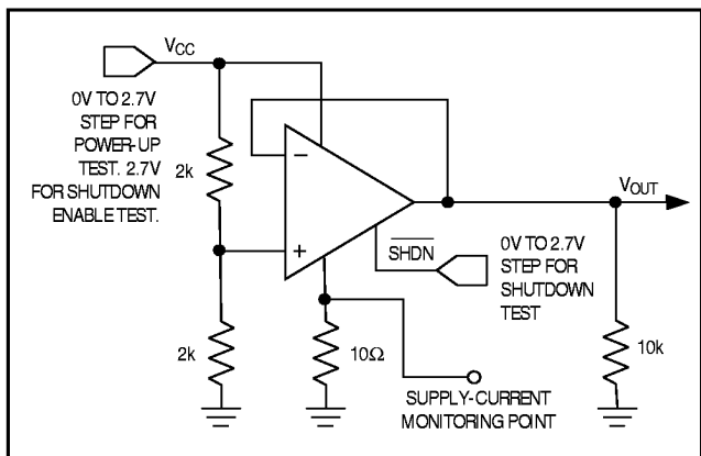
Figure 10. Power-Up/Shutdown Test Circuit
