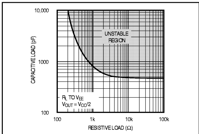
Figure 4. Capacitive-Load Stability
