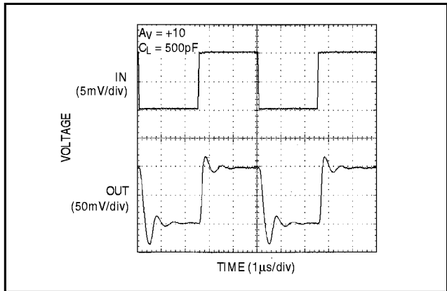
Figure 6. MAX4124/25/28 Small-Signal Transient Response with Capacitive Load
