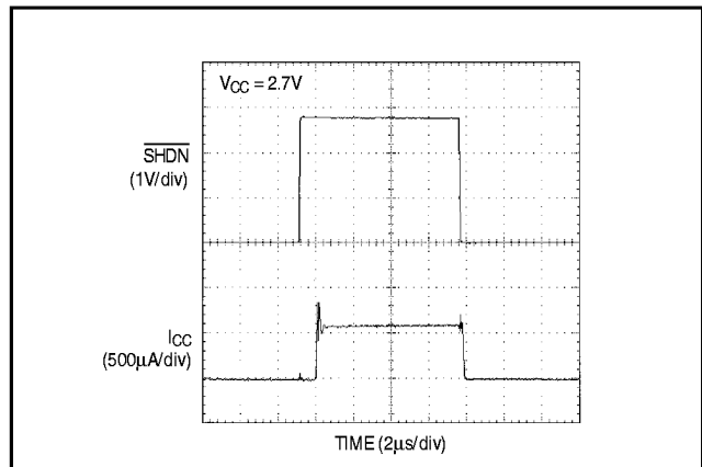
Figure 14. Shutdown Enable/Disable Supply Current
