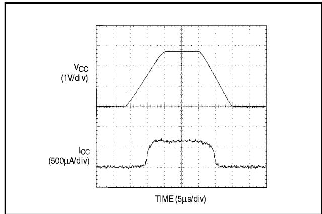
Figure 12. Power-Up Supply Current
