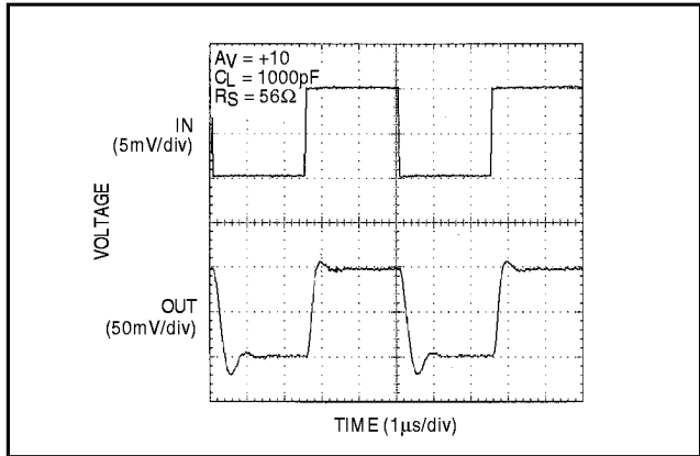
Figure 8. MAX4124/25/28 Transient Response to Capacitive Load with Isolation Resistor
