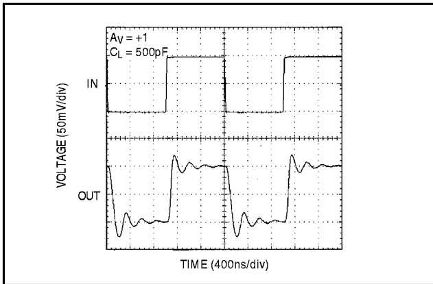
Figure 5. MAX4122/23/26/27/29 Small-Signal Transient Response with Capacitive Load
