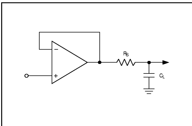
Figure 9. Capacitive-Load-Driving Circuit
