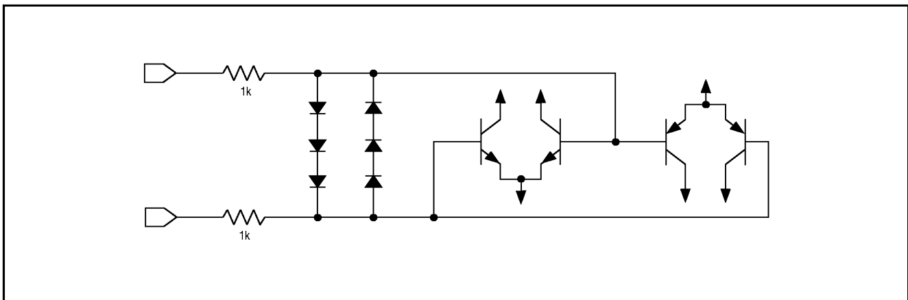
Figure 2. Input Protection Circuit
