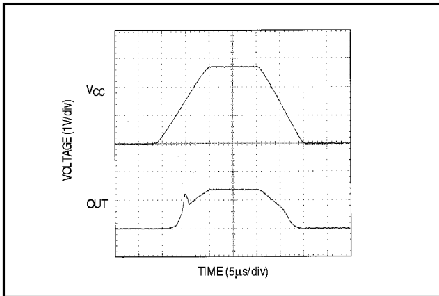
Figure 11. Power-Up Output Voltage
