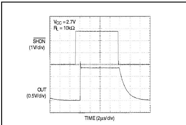
Figure 13. Shutdown Output Voltage
