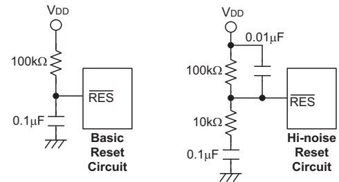
Reset Circuit
