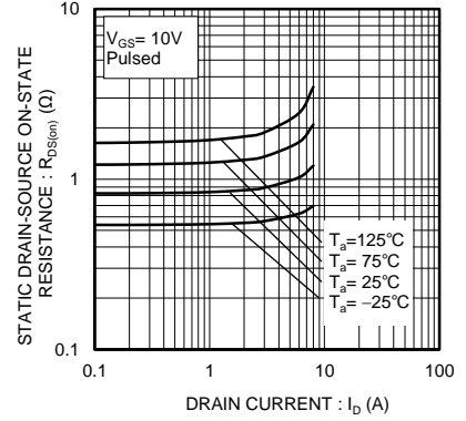
Fig.6 Static Drain-Source On-State Resistance vs. Drain Current
