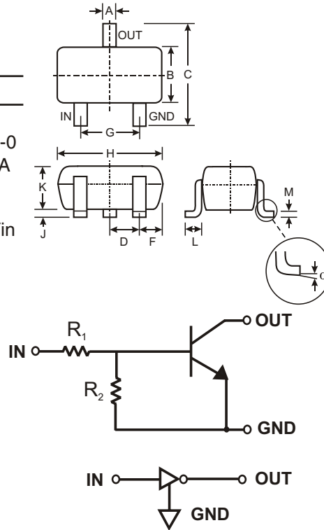
SCHEMATIC DIAGRAM
