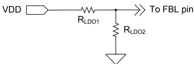
Figure 9 — LDO Start-Up
