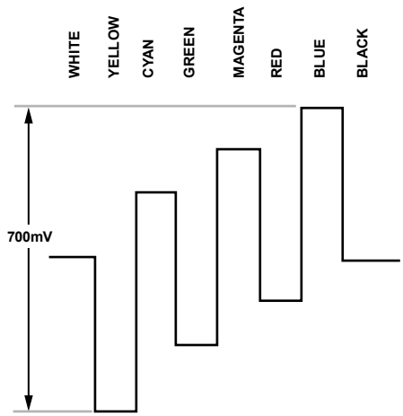
Figure 116. Pb Levels—NTSC
