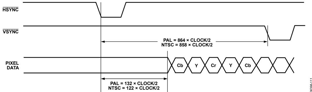
Figure 110. SD Timing Mode 2 Odd-to-Even Field Transition (Master/Slave)
