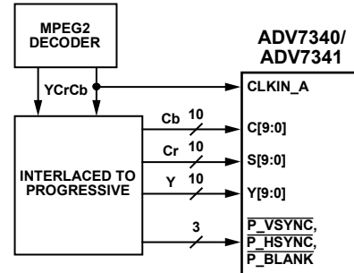
Figure 54. ED/HD Only Example Application
