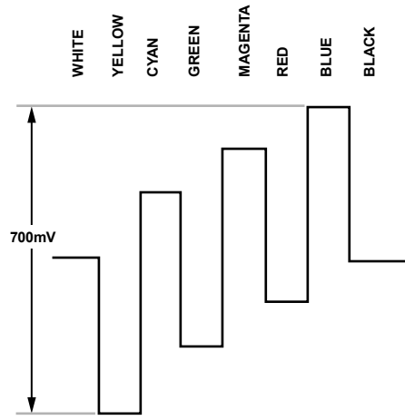
Figure 119. Pb Levels—PAL
