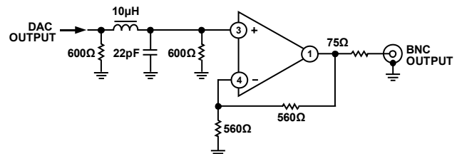
Figure 84. Example of Output Filter for SD, 16 \times Oversampling
