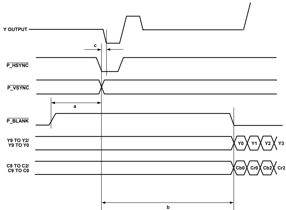
Figure 15. ED-DDR, 8-/10-Bit, 4:2:2 YCrCb ( \overline{\text{HSYNC}}/\overline{\text{VSYNC}} ) Input Timing Diagram
