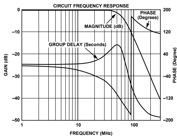
Figure 89. Output Filter Plot for HD, 4x Oversampling
