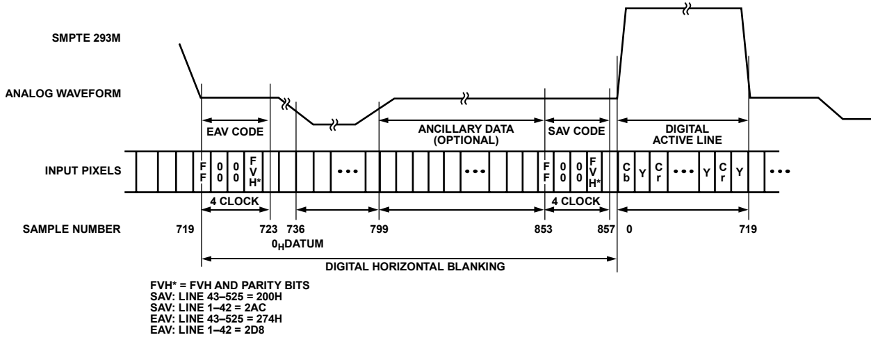
Figure 135. EAV/SAV Input Data Timing Diagram (SMPT 293M)
