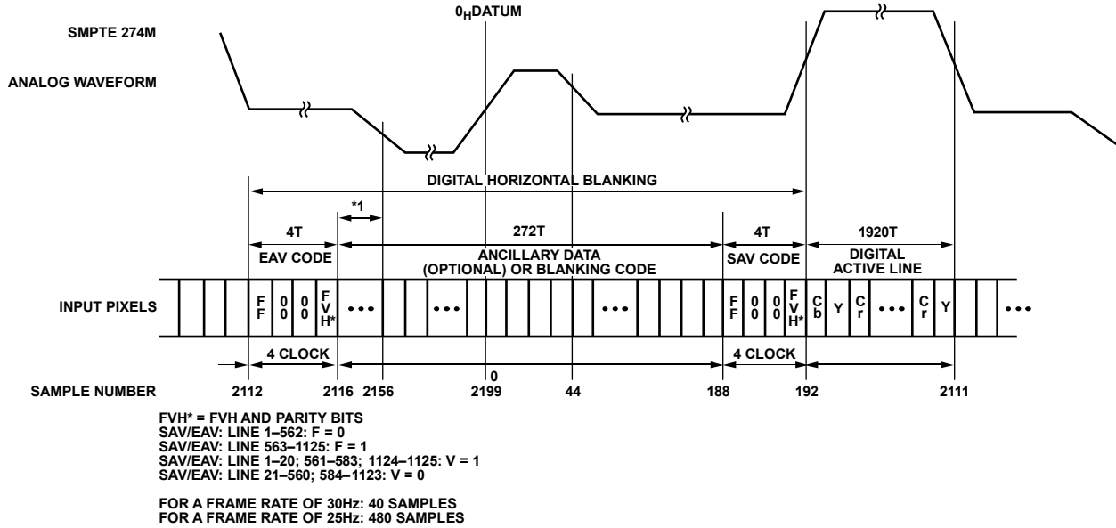
Figure 134. EAV/SAV Input Data Timing Diagram (SMPT 274M)
