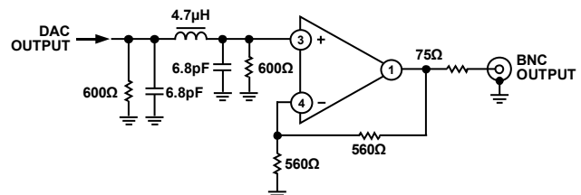
Figure 85. Example of Output Filter for ED, 8 \times Oversampling
