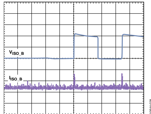
Figure 28. Battery Detection Waveform, VSYSTEM[2:0] = 000 (Binary) = 4.3 V, No Battery
