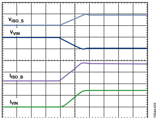
Figure 25. Input Current-Limit Transition from 100 mA to 900 mA, ISO_Sx Load = 66 \Omega , Charging = 750 mA
