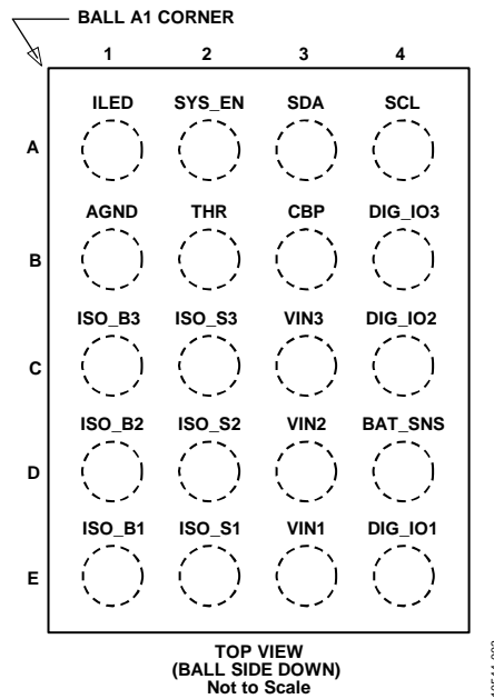
Figure 3. Pin Configuration
