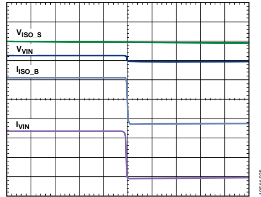
Figure 26. VBUS Disconnect
