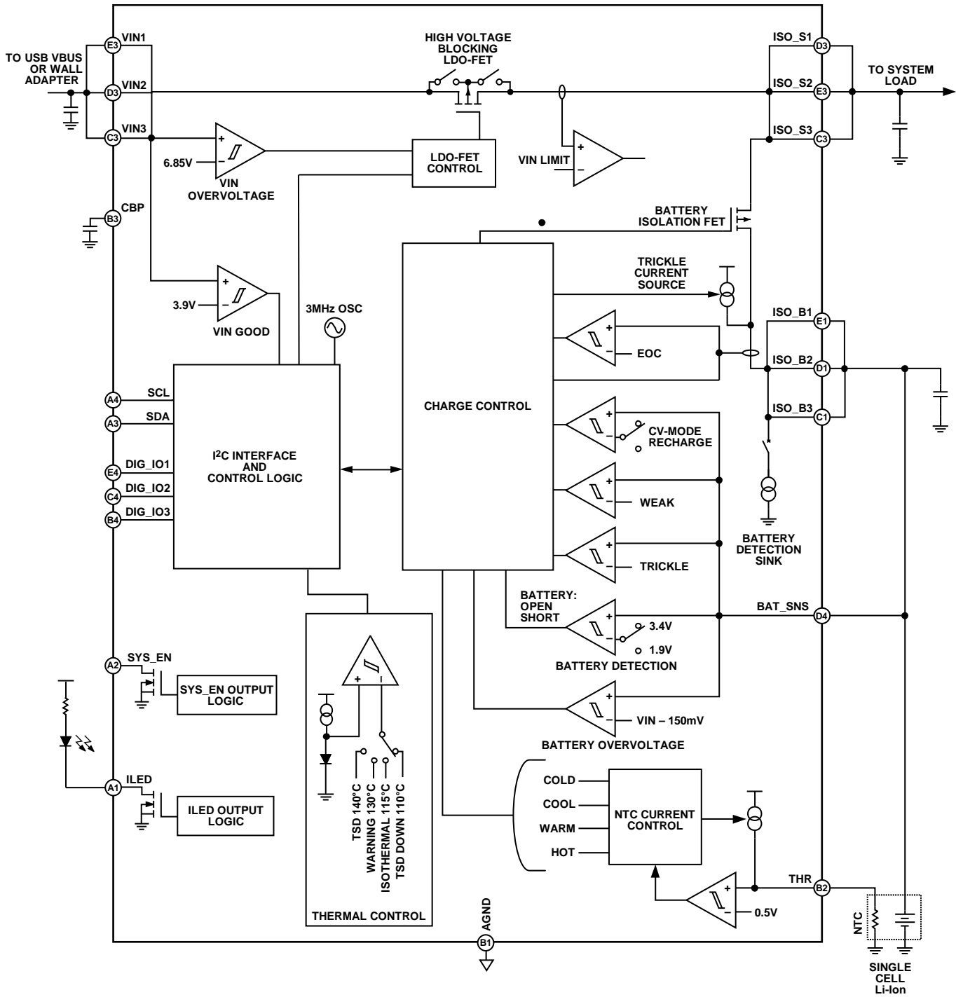
Figure 29. Block Diagram
