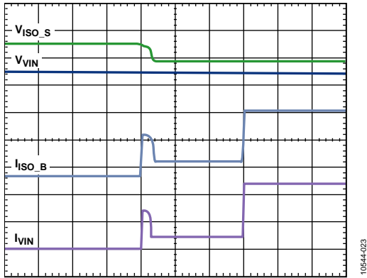
Figure 23. Charging Start-up, V_{VIN} = 5.0\text{ V} , ILIM[3:0] = 0110 (Binary) = 500 mA, ICHG[4:0] = 01110 (Binary) = 750 mA
