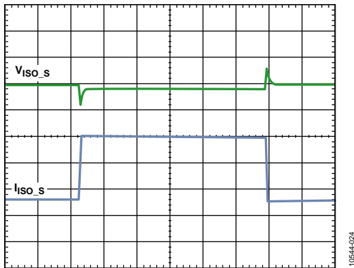
Figure 24. Load Transient, I_{ISO_Sx} Load = 300 mA to 1500 mA to 300 mA
