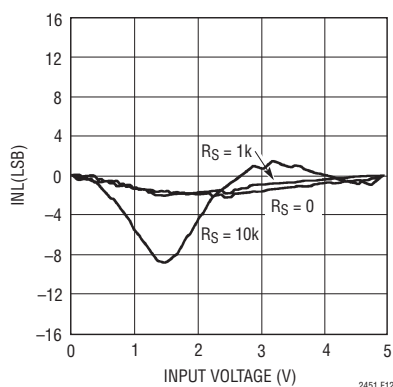
Figure 12. Measured INL vs Input Voltage, C_{IN} = 0.1\mu\text{F} , V_{CC} = 5\text{V} , T_A = 25^\circ\text{C}
