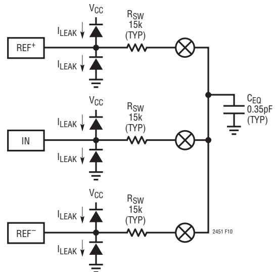
Figure 10. LTC2451 Analog Input and Reference Pins Equivalent Circuit
