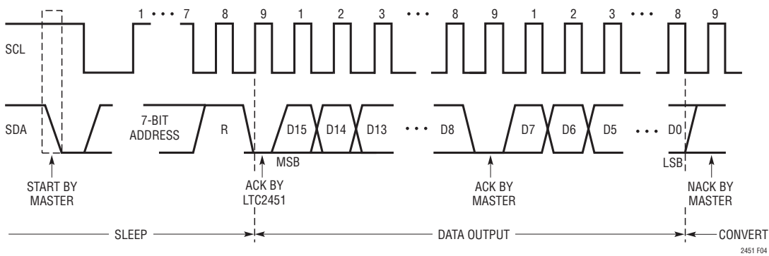
Figure 4. Timing Diagram for Read Sequence
