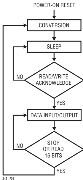
Figure 1. State Diagram
