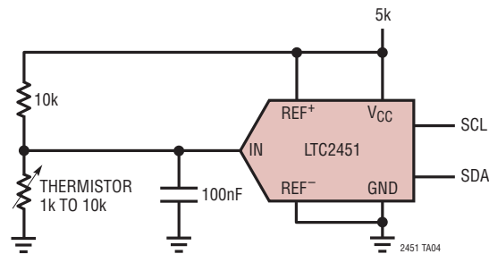
Thermistor Measurement
