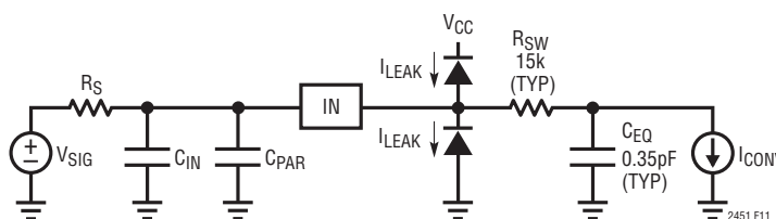
Figure 11. LTC2451 Input Drive Equivalent Circuit
