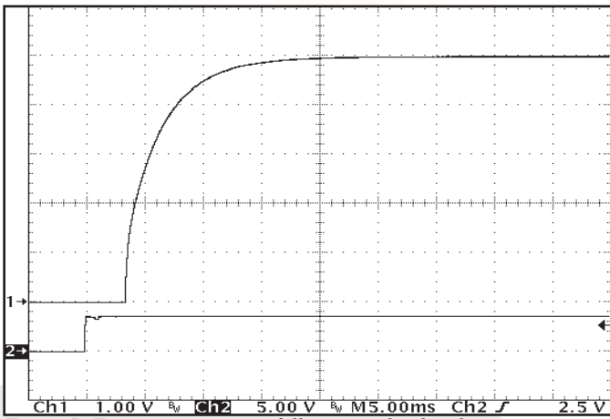
Figure 7: Turn-on transient at full resistive load and zero output capacitance initiated by ENA1. Input voltage pre-applied. Ch 1: Vout (1V/div). Ch 2: ENA1 (5V/div).
