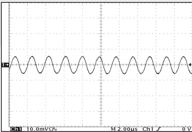
Figure 15: Input terminal current ripple, i_c , at full rated output current and nominal input voltage with SynQor MQ filter module (50mA/div). Bandwidth: 20MHz. See Figure 14.
